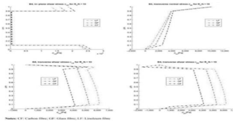
Figure 4 Stress components through the thickness of the sandwich spherical shell embedding composite skins (B4) with Ra/h = 10
